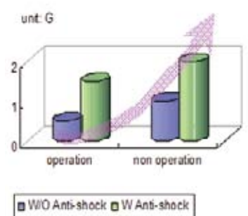
Vibration Test
